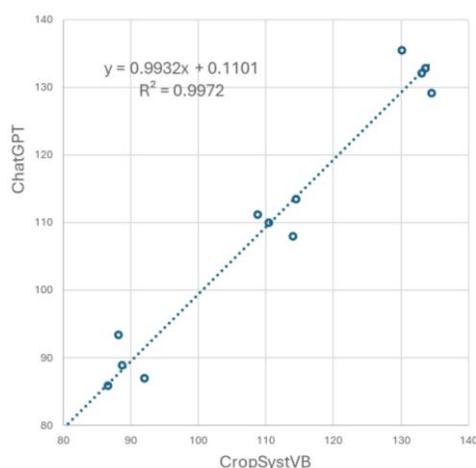
Figure 1. Example results of ChatGPT irrigation decisions (on the Y-axis) for a loam soil with a field capacity of 0.26 m^3 m^{-3} and a wilting point of 0.12 m^3 m^{-3} , compared with the results of a dynamic mechanistic crop model (CropSystVB), on the X-axis. The graph shows that ChatGPT irrigations were mostly applied on the same day as predicted by CropSystVB, with a few exceptions with one-day difference. In addition to the data shown in the Figure, there are six data points with both ChatGPT and CropSystVB showing zero irrigation.
