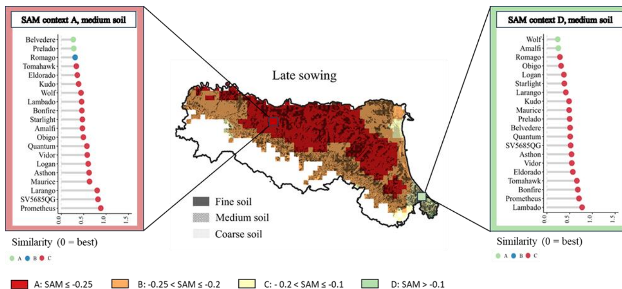
Figure 1. Central panel: example of the agro-climatic characterization of the study area obtained by clustering the Synthetic Agroclimatic Index (SAM, normalized difference of rainfall and reference evapotranspiration during the cropping season) calculated for late sowings. Negative SAM values indicate dry climates while positive values highlight humid conditions. Left and right panels show two examples of cultivar ranking obtained for different conditions, humid (right panel) and dry (left panel). In the ranking, green points indicate recommended, blue represents second-choice varieties, and red highlights less suitable varieties.
