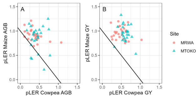
Figure 1. Maize and cowpea pLER for aboveground biomass (AGB)(A) and grain yield (B) as simulated by the STICS model for twenty-six historical growing seasons (1996-2021) for Murewa and Mutoko districts. In all subplots, the black solid line is LER = 1. Two outliers (> 1.5) were removed for the pLER of cowpea grain yield.
