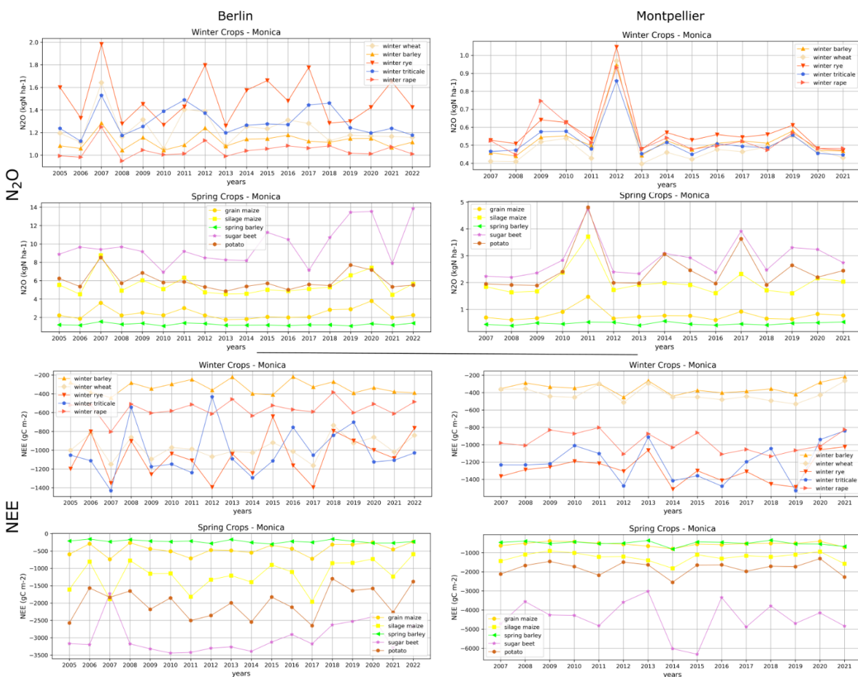
Figure 1. N 2 O emission and NEE, obtained using MONICA, for winter and spring crops in arable zone around the metropolis Berlin (Crops in Brandenburg) and Montpellier (Crops in Occitania), from 2005 to 2022 for Berlin and 2007 to 2021 for Montpellier.
