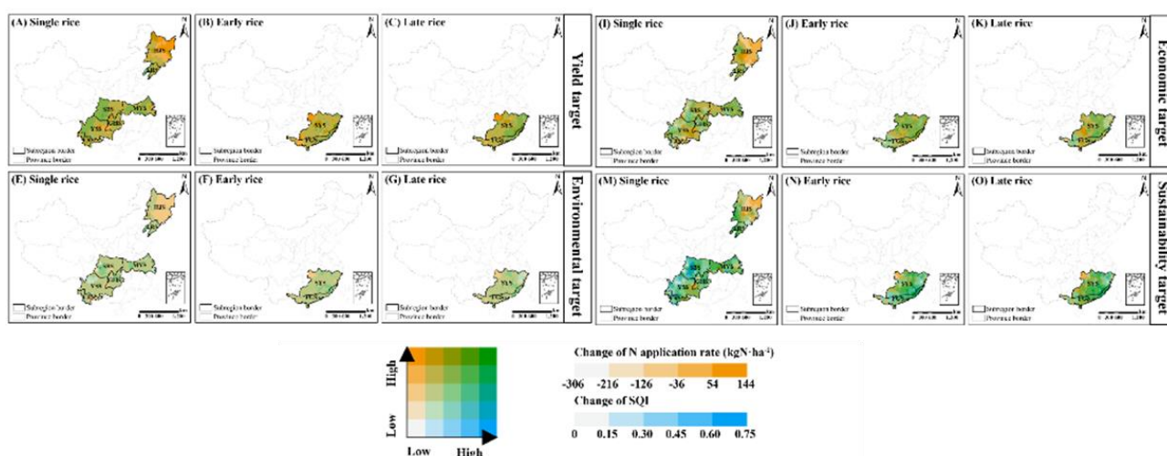
Figure 2. Change of N application rate and soil quality for achieving yield, environmental, economic and sustainability targets
