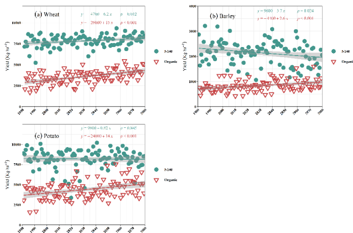
Figure 1. Simulated wheat, barley and potato yield under organic and optimal conventional fertilizer rate at long term conditions
